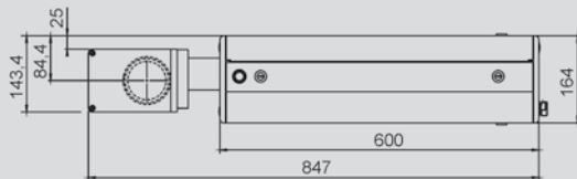
Laser head with standard scan head and lens
